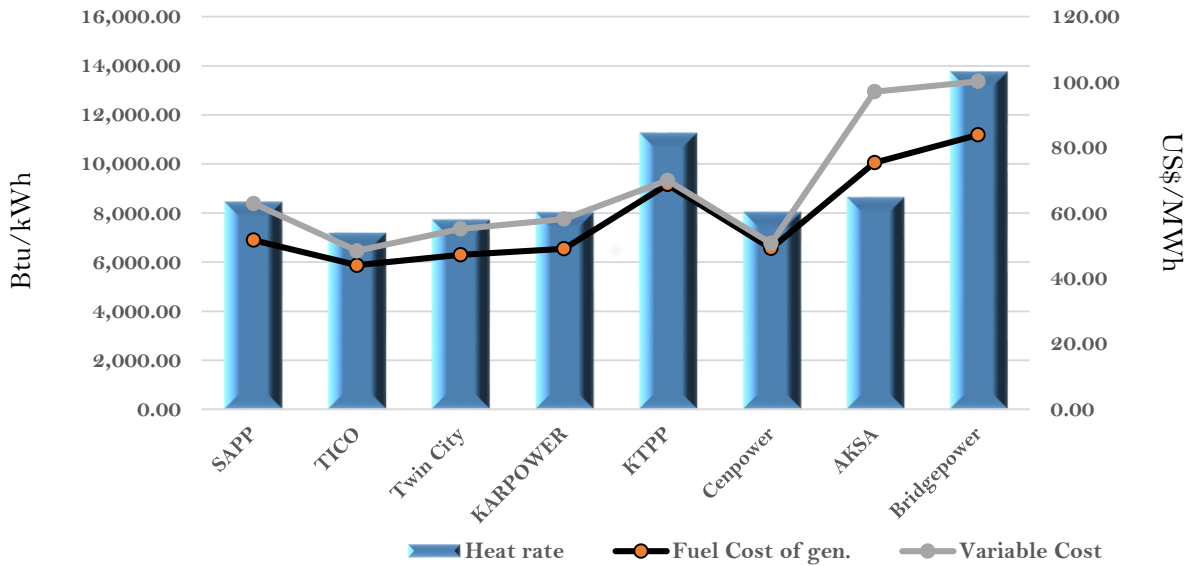
Efficiency and fuel cost of generation on the 3rd December 2023
