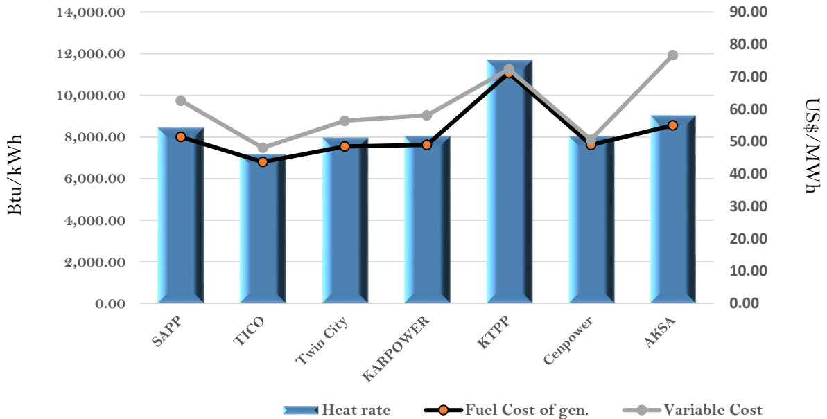
Efficiency and fuel cost of generation on the 3rd December 2023
