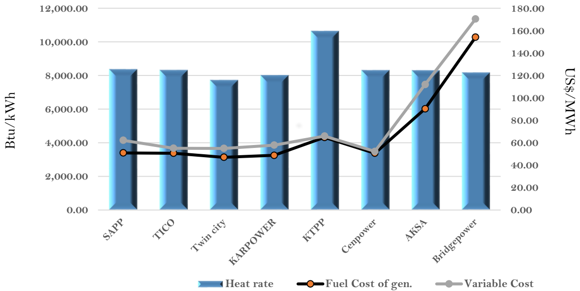
Efficiency and fuel cost of generation on the 12th December 2023
