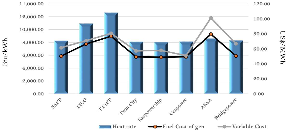
Efficiency and fuel cost of generation on the 21st December 2023
