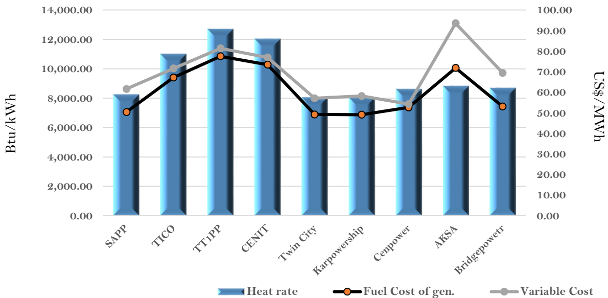
Efficiency and fuel cost of generation on the 21st December 2023
