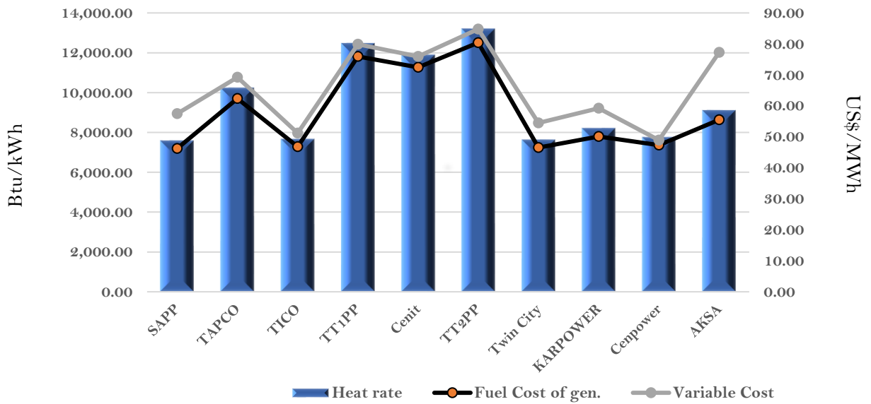
Efficiency and fuel cost of generation on the 14th August 2022
