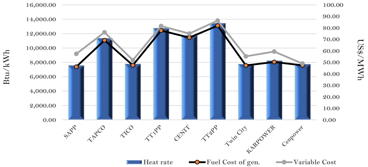
Efficiency and fuel cost of generation on the 13th August 2022
