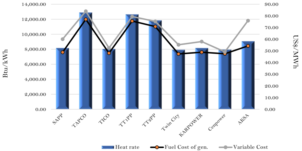
Efficiency and fuel cost of generation on the 14th December 2022
