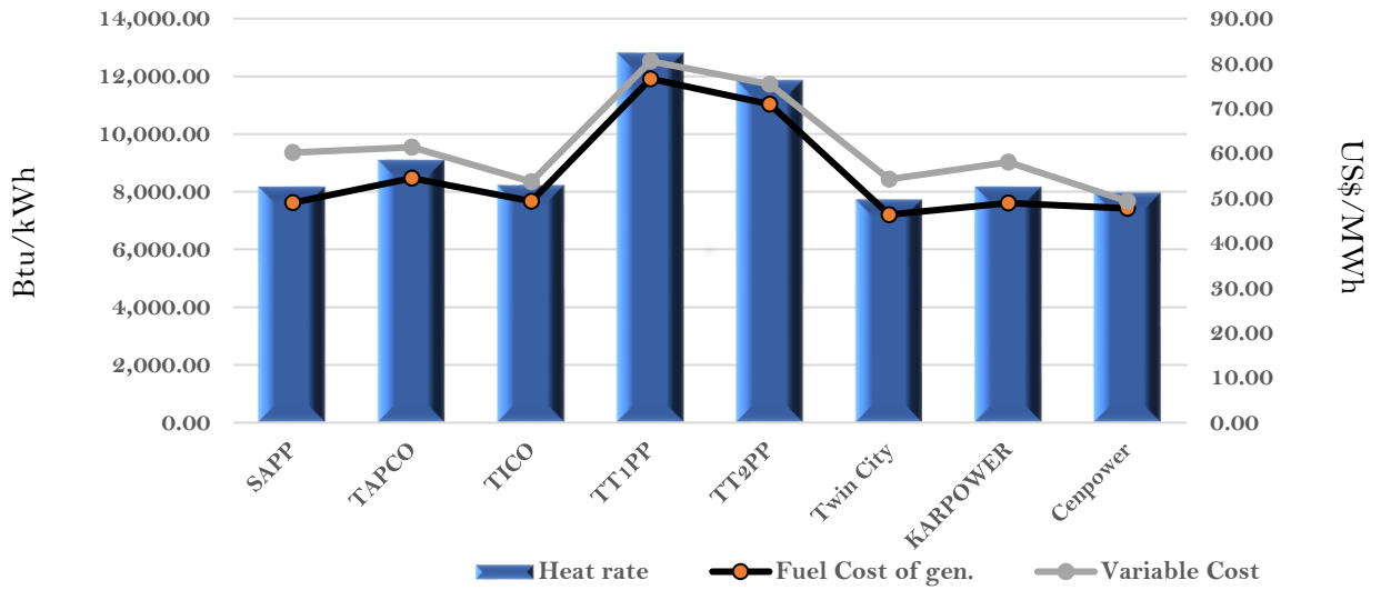
Efficiency and fuel cost of generation on the 13th December 2022
