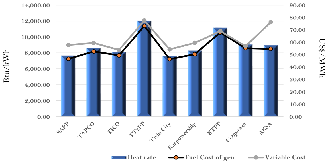
Efficiency and fuel cost of generation on the 21st July 2022
