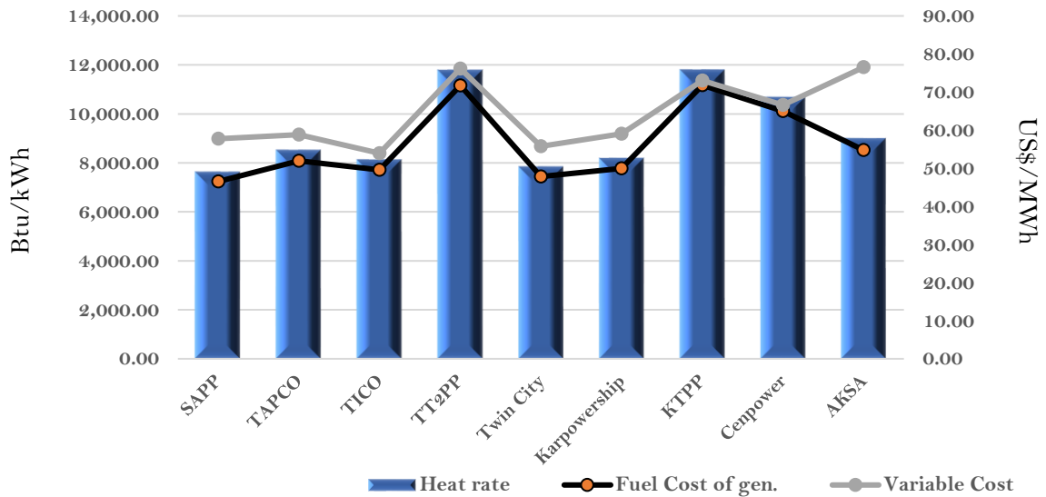
Efficiency and fuel cost of generation on the 21st July 2022
