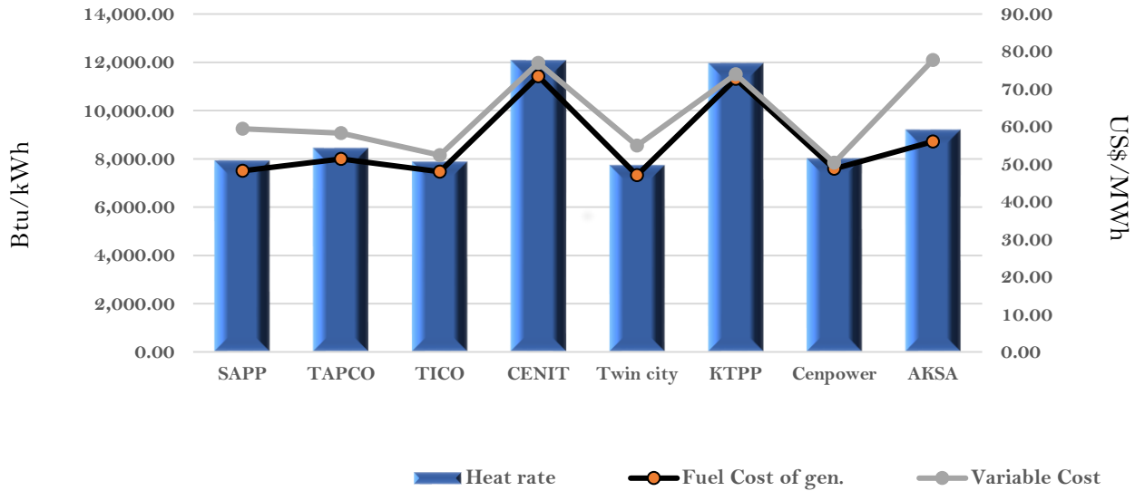
Efficiency and fuel cost of generation on the 31st July 2022
