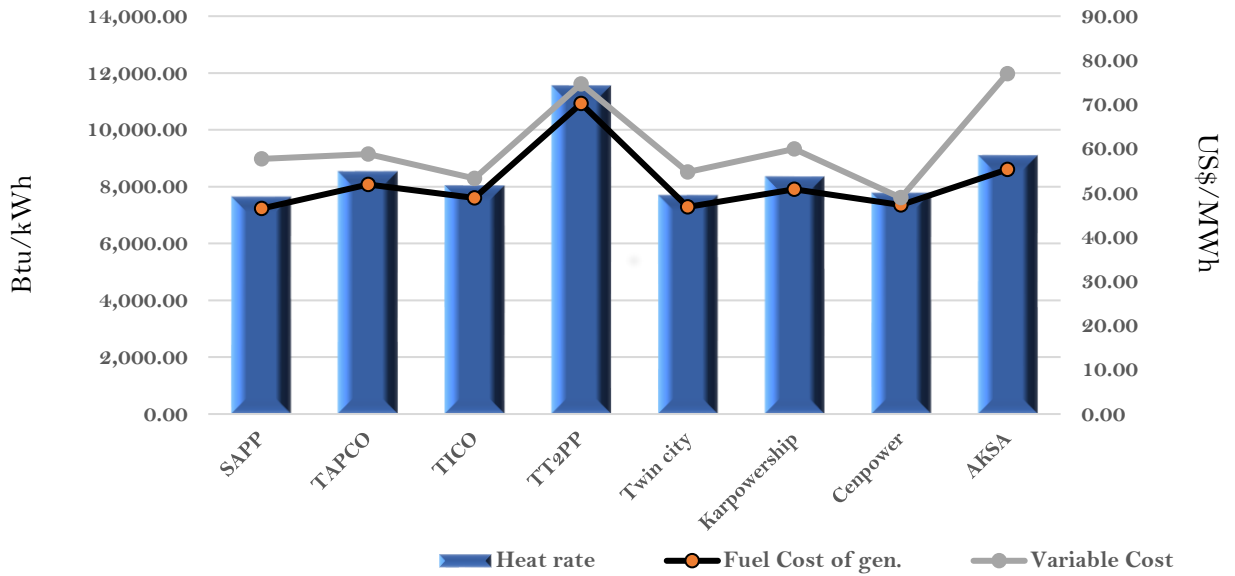
Efficiency and fuel cost of generation on the 29th July 2022
