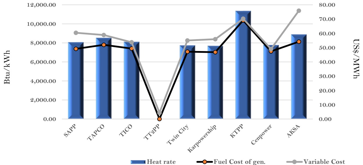
Efficiency and fuel cost of generation on the 26th July 2022
