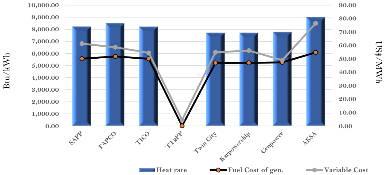
Efficiency and fuel cost of generation on the 25th July 2022
