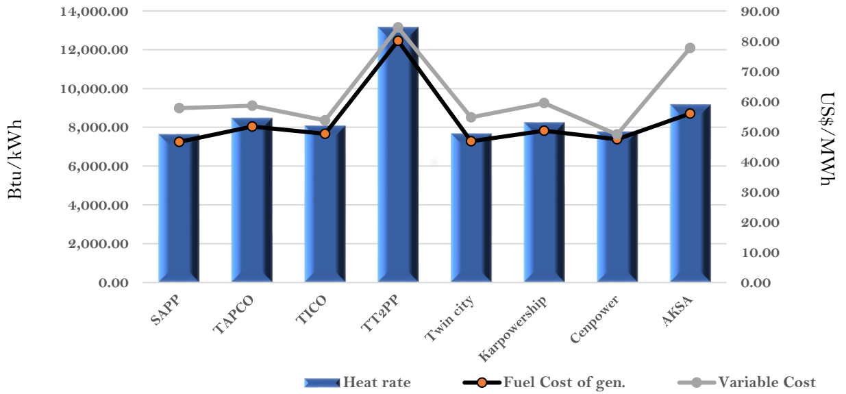
Efficiency and fuel cost of generation on the 30th July 2022
