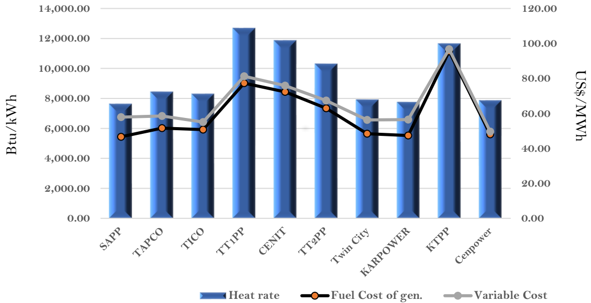
Efficiency and fuel cost of generation on the 14th June 2022
