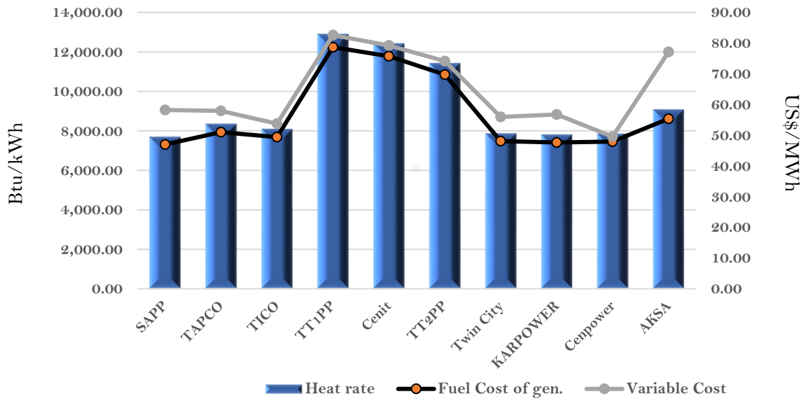
Efficiency and fuel cost of generation on the 14th June 2022
