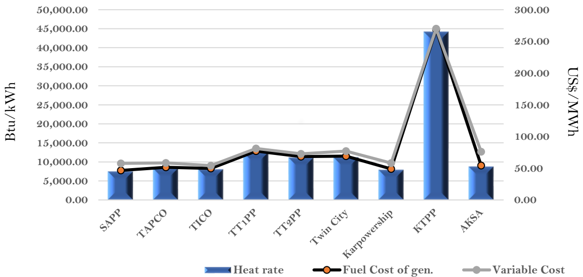
Efficiency and fuel cost of generation on the 21st June 2022
