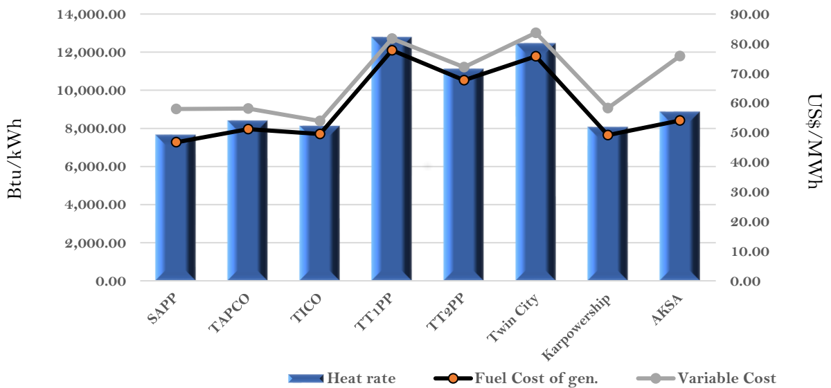
Efficiency and fuel cost of generation on the 19th June 2022
