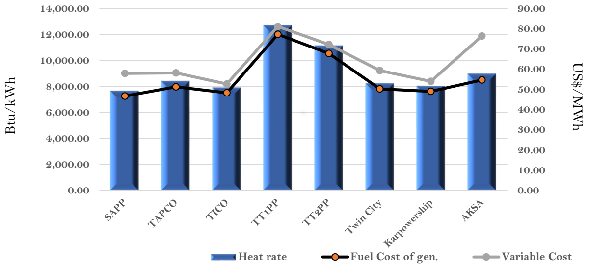
Efficiency and fuel cost of generation on the 18th June 2022
