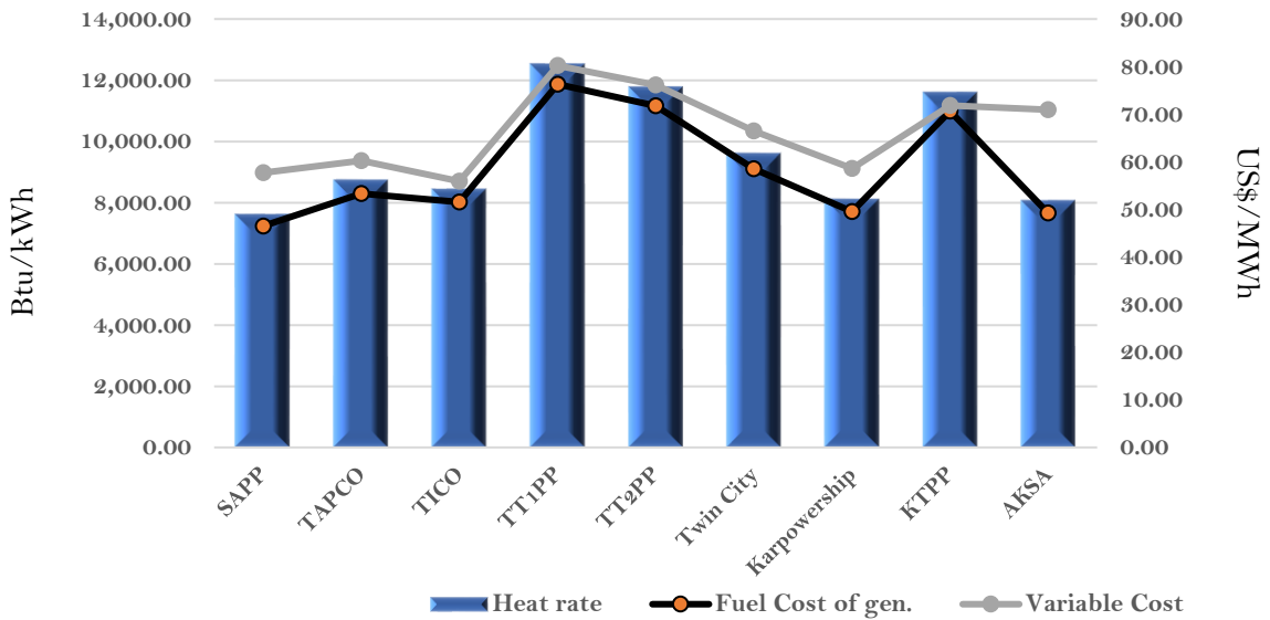
Efficiency and fuel cost of generation on the 20th June 2022
