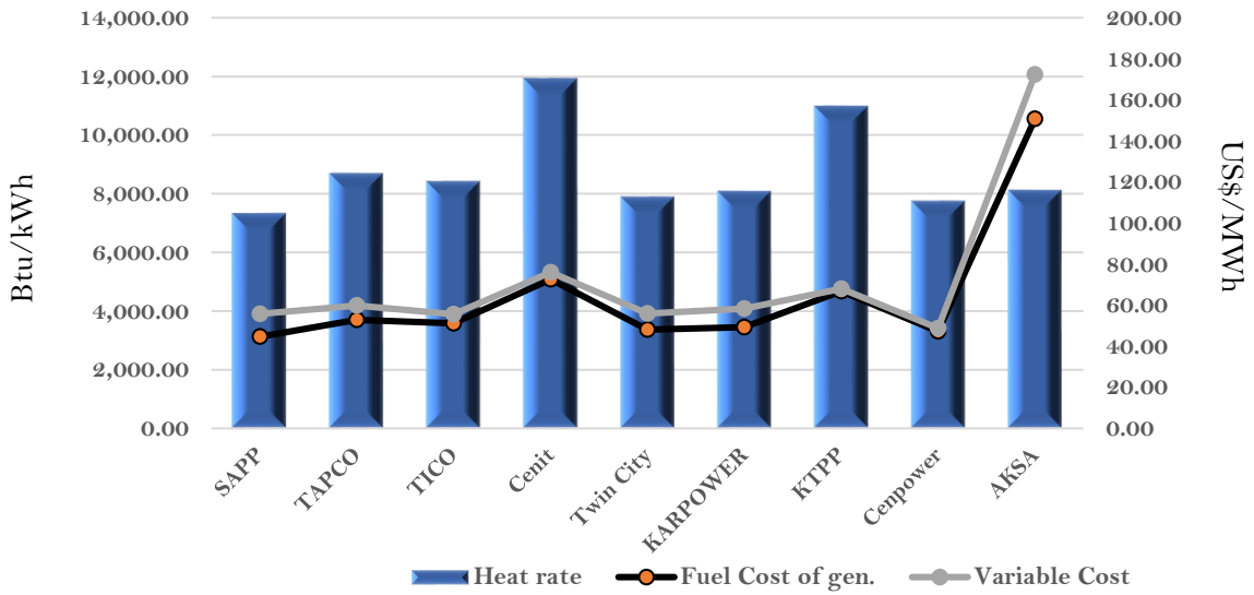
Efficiency and fuel cost of generation on the 14th March 2022
