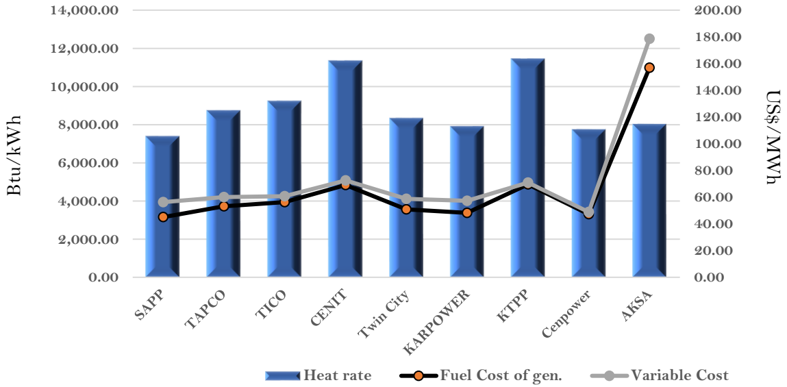
Efficiency and fuel cost of generation on the 14th March 2022
