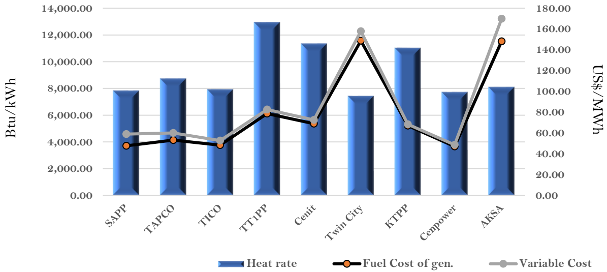
Efficiency and fuel cost of generation on the 18th March 2022
