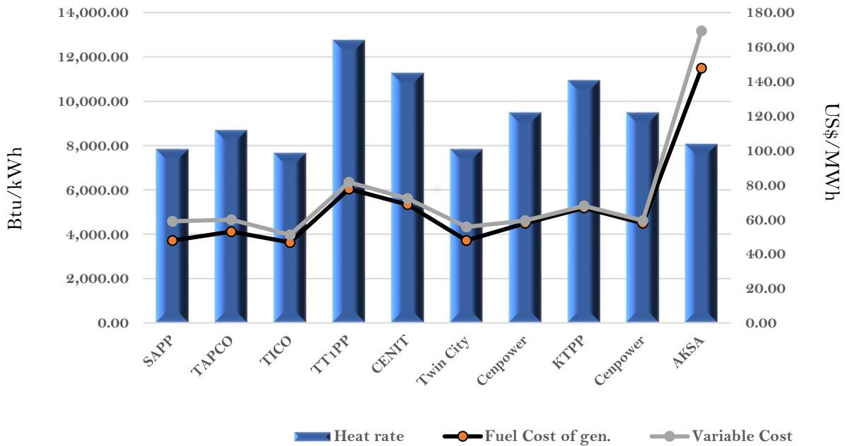
Efficiency and fuel cost of generation on the 19th March 2022
