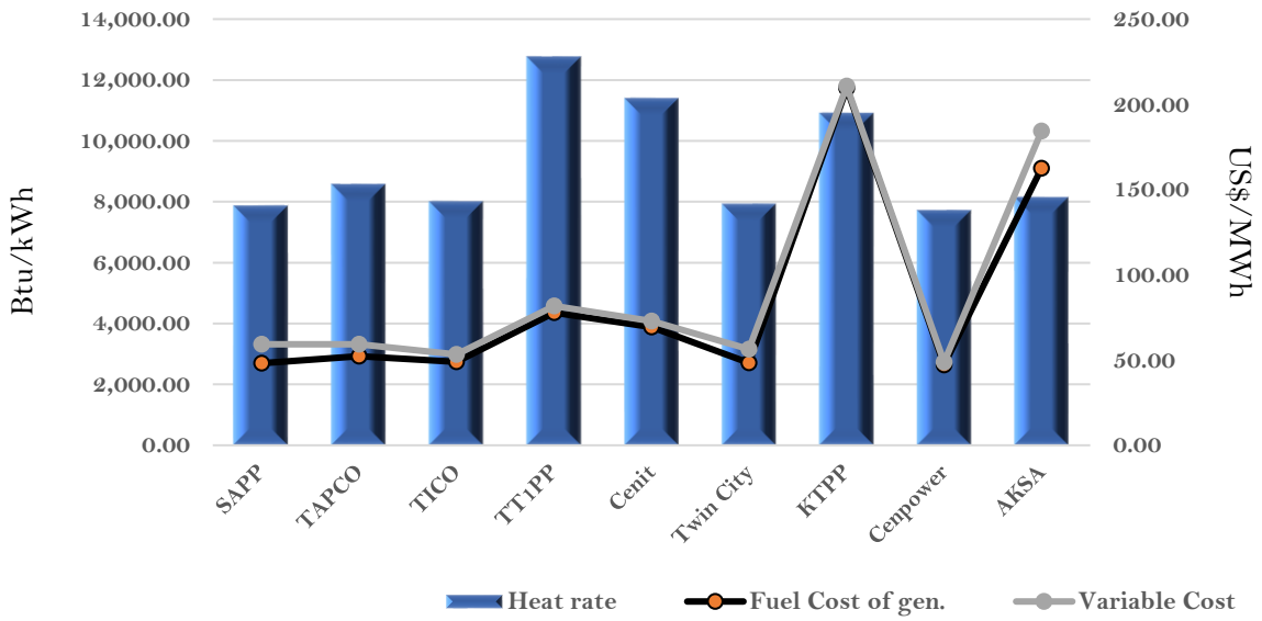
Efficiency and fuel cost of generation on the 28th March 2022
