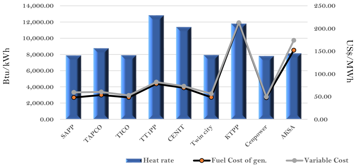
Efficiency and fuel cost of generation on the 28th March 2022
