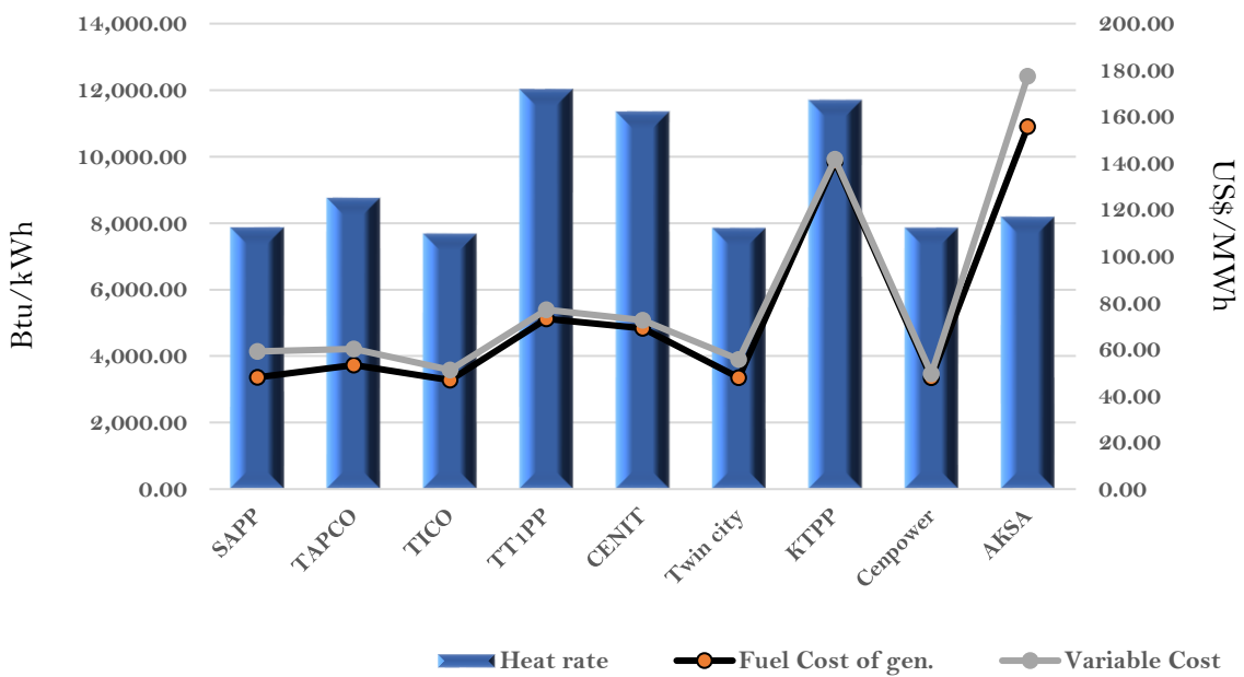
Efficiency and fuel cost of generation on the 30th March 2022
