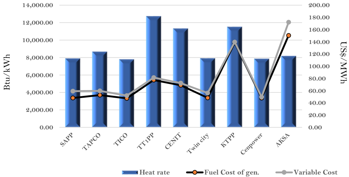
Efficiency and fuel cost of generation on the 30th March 2022
