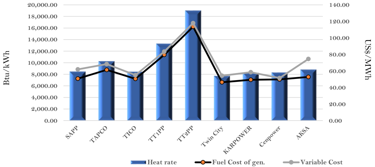
Efficiency and fuel cost of generation on the 2nd November 2022
