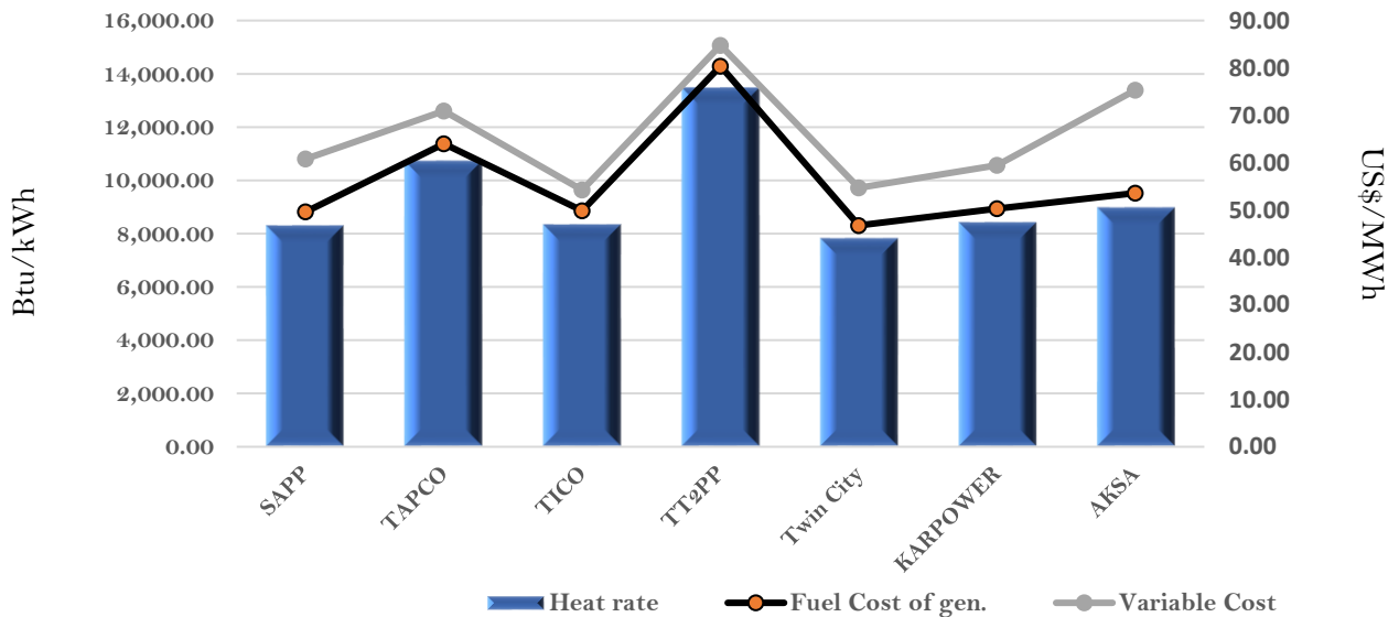
Efficiency and fuel cost of generation on the 3rd November 2022
