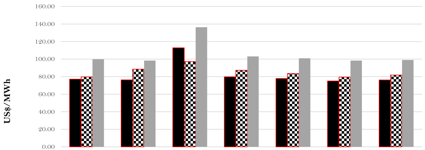
System Marginal Cost Vs Average Market Prices for Week 1 of September 2022
