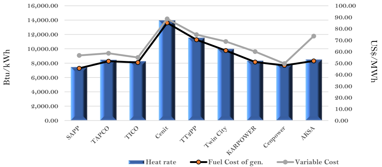
Efficiency and fuel cost of generation on the 14th September 2022
