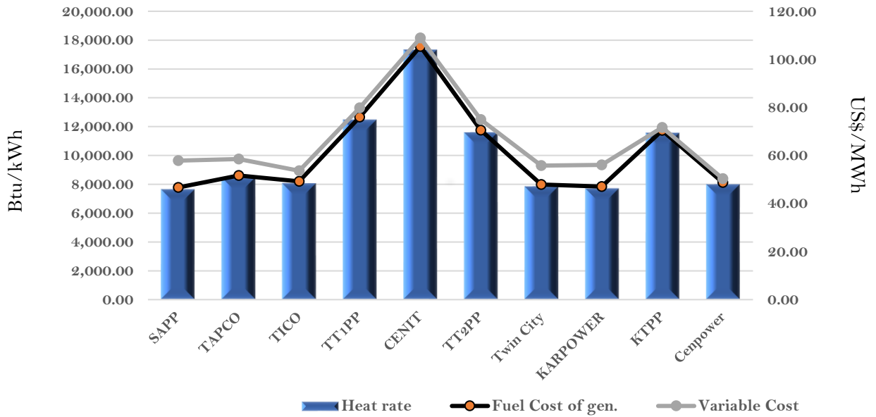
Efficiency and fuel cost of generation on the 13th September 2022
