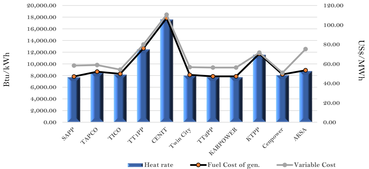
Efficiency and fuel cost of generation on the 12th September 2022
