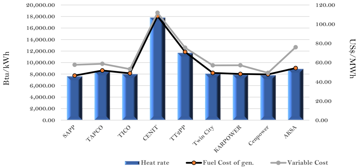
Efficiency and fuel cost of generation on the 11th September 2022
