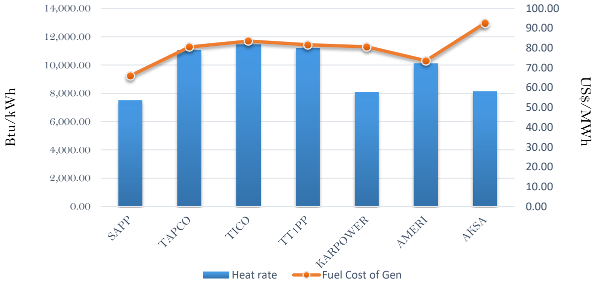
Efficiency and fuel cost of generation on the 1st December 2018
