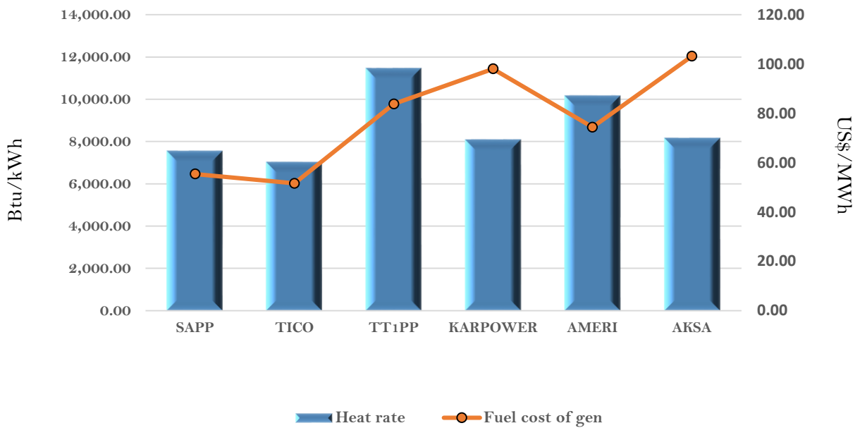
Efficiency and fuel cost of generation on the 5th April 2018
