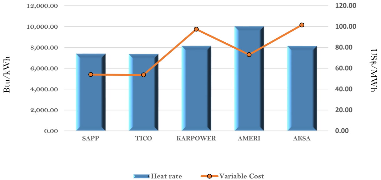
Efficiency and fuel cost of generation on the 4th April 2018
