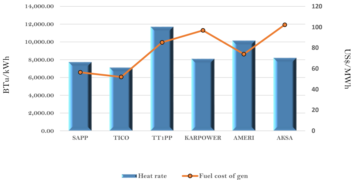
Efficiency and fuel cost of generation on the 6th April 2018
