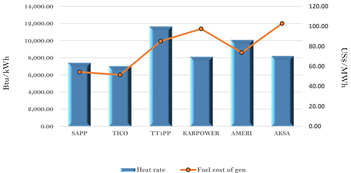
Efficiency and fuel cost of generation on the 4th April 2018
