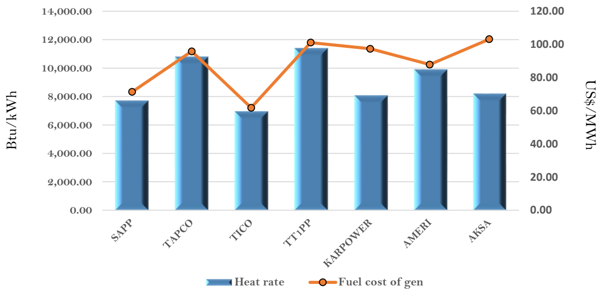
Estimated Efficiency and fuel cost of generation on the 29th March 2018
