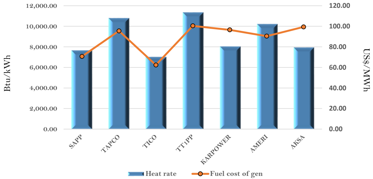
Estimated Efficiency and fuel cost of generation on the 28th March 2018
