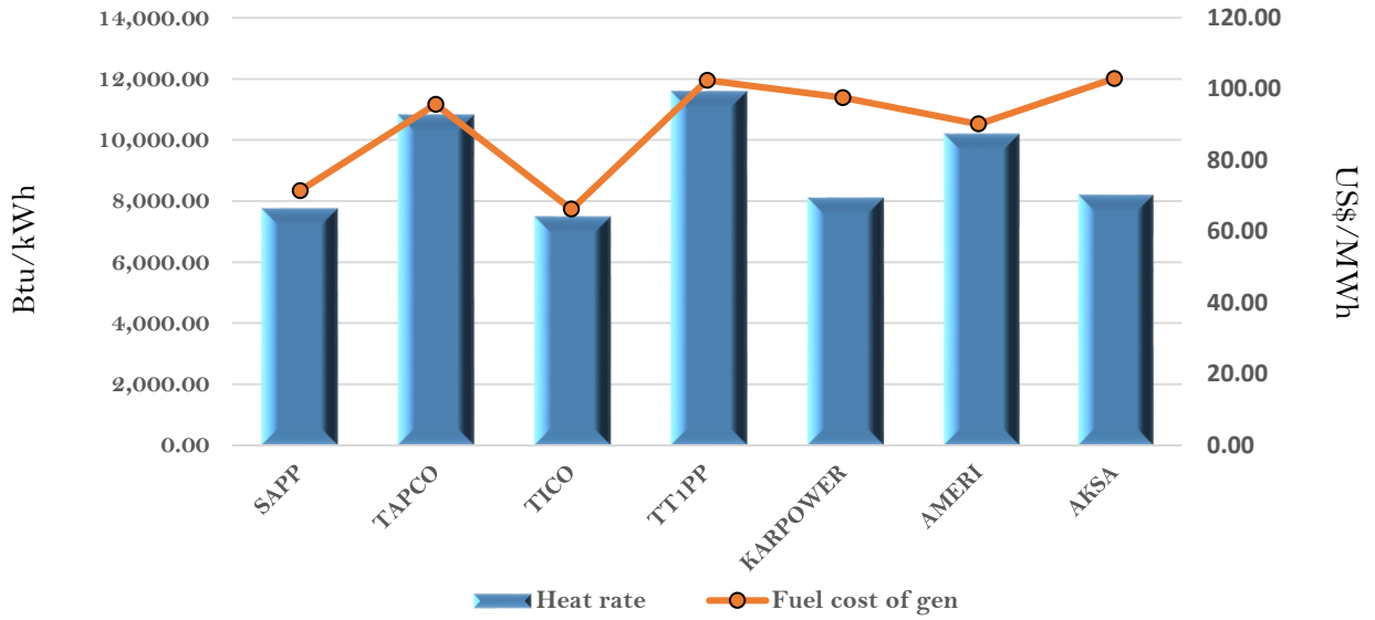
Estimated Efficiency and fuel cost of generation on the 22th March 2018
