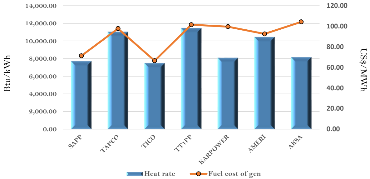
Estimated Efficiency and fuel cost of generation on the 24th March 2018
