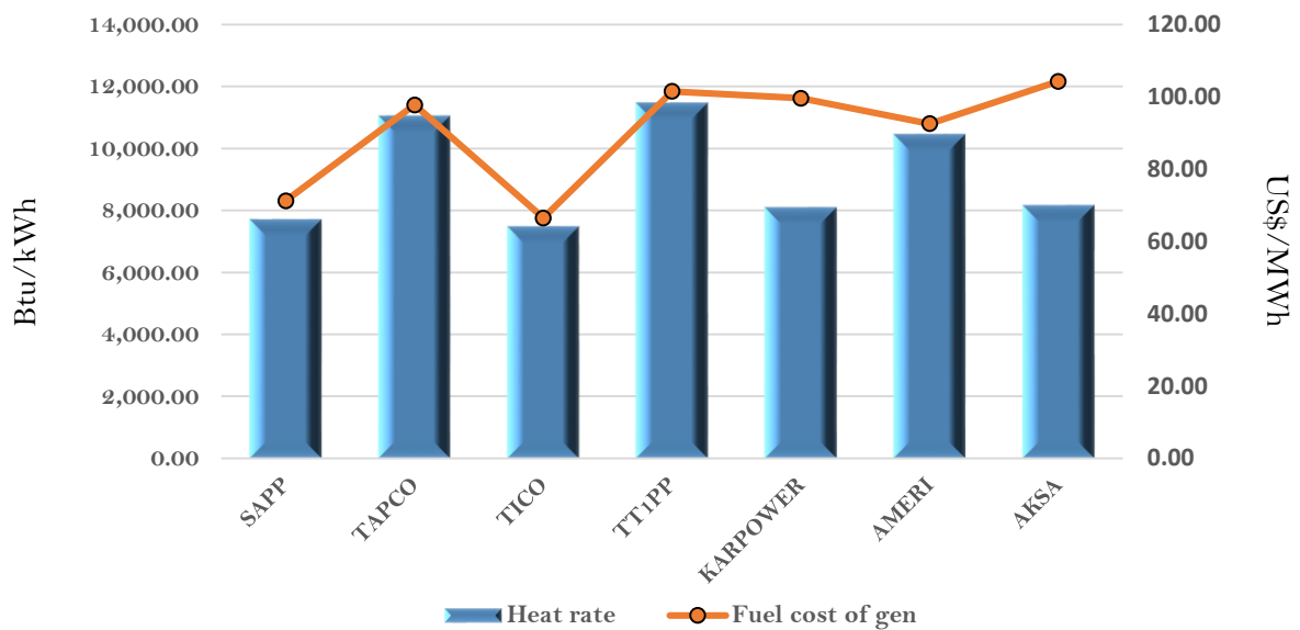
Estimated Efficiency and fuel cost of generation on the 25th March 2018
