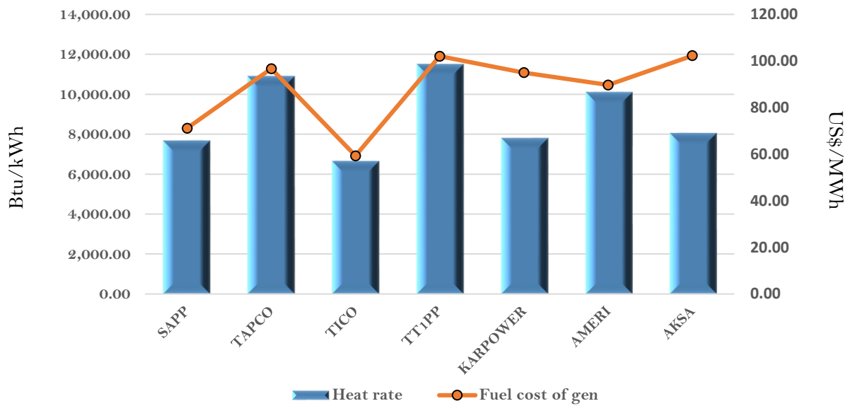
Estimated Efficiency and fuel cost of generation on the 27th March 2018
