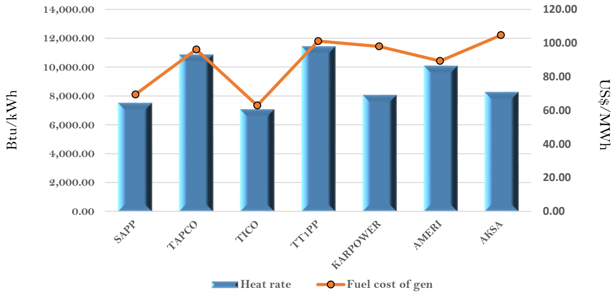
Estimated Efficiency and fuel cost of generation on the 26th March 2018
