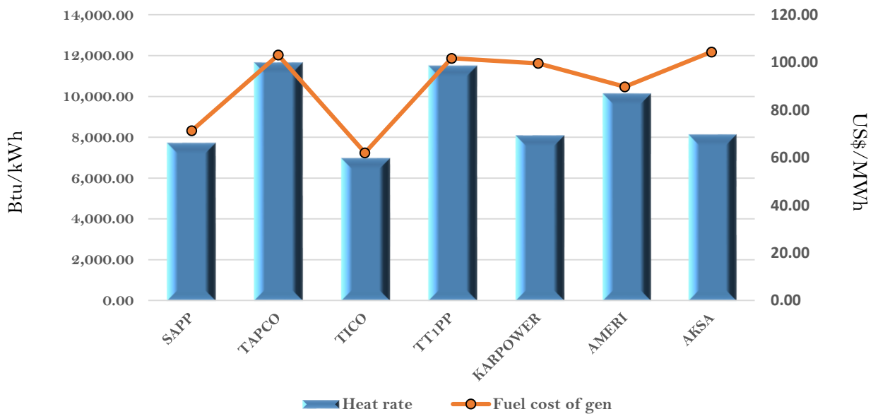
Estimated Efficiency and fuel cost of generation on the 23th March 2018
