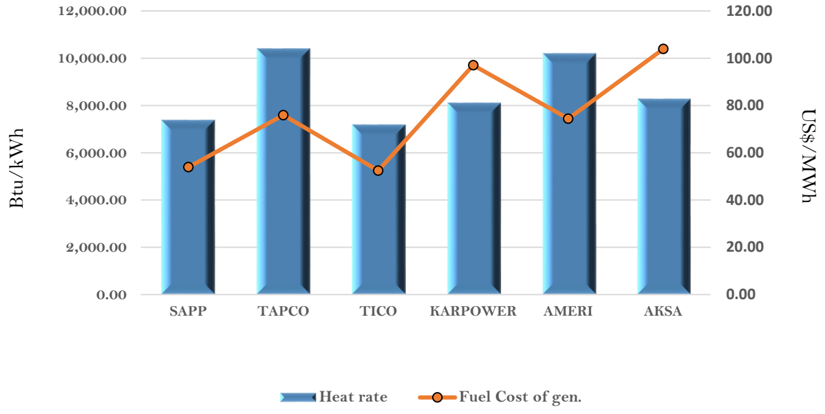
Efficiency and fuel cost of generation on the 27th May 2018
