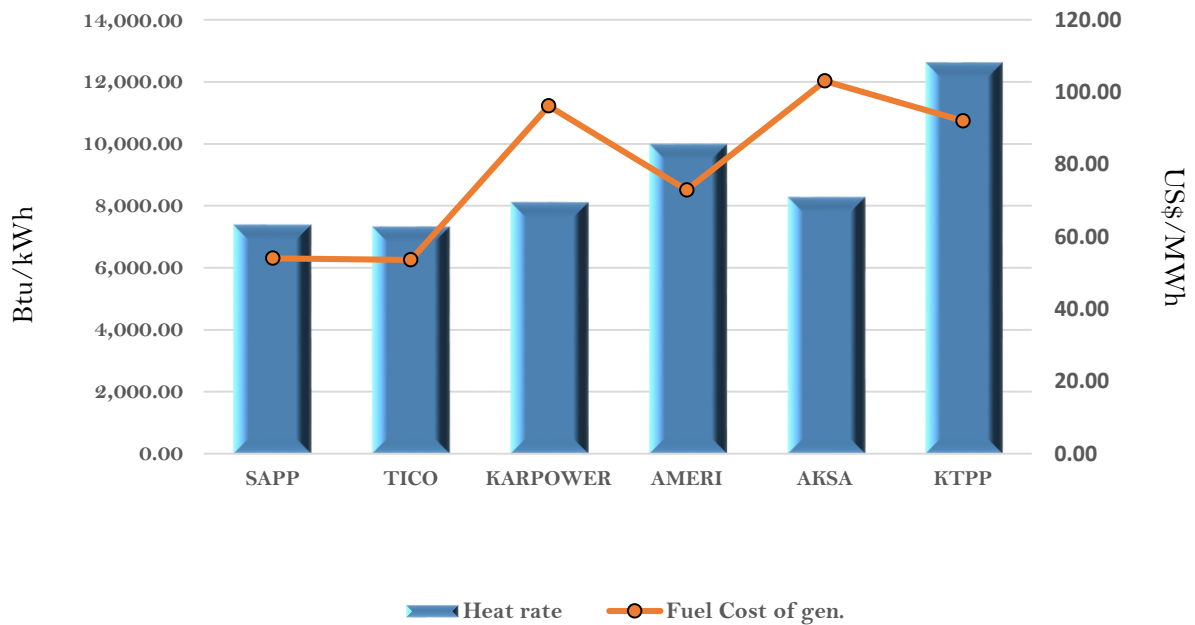
Efficiency and fuel cost of generation on the 29th May 2018
