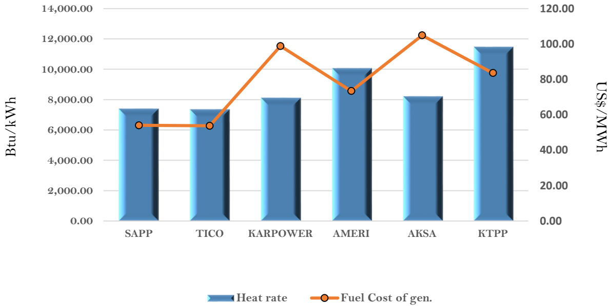
Efficiency and fuel cost of generation on the 31st May 2018
