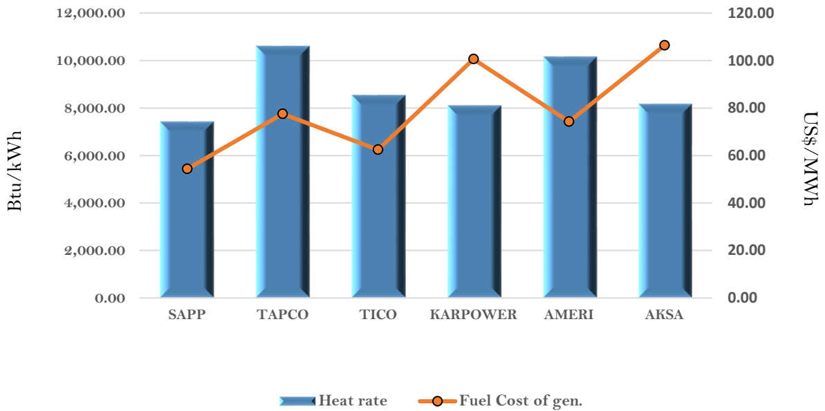
Efficiency and fuel cost of generation on the 22nd May 2018
