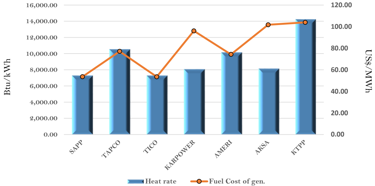
Efficiency and fuel cost of generation on the 29th May 2018
