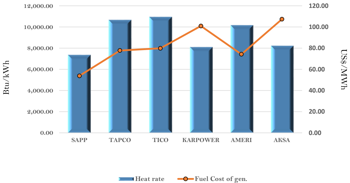
Efficiency and fuel cost of generation on the 23rd May 2018
