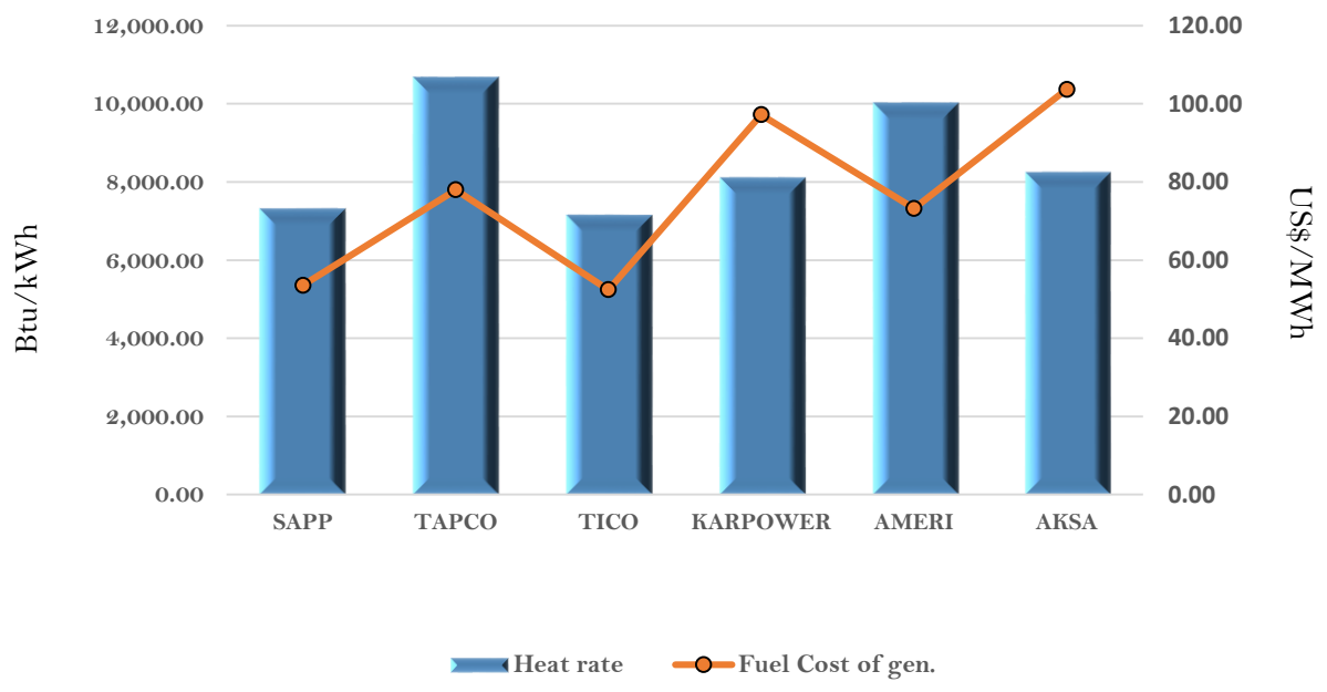
Efficiency and fuel cost of generation on the 27th May 2018
