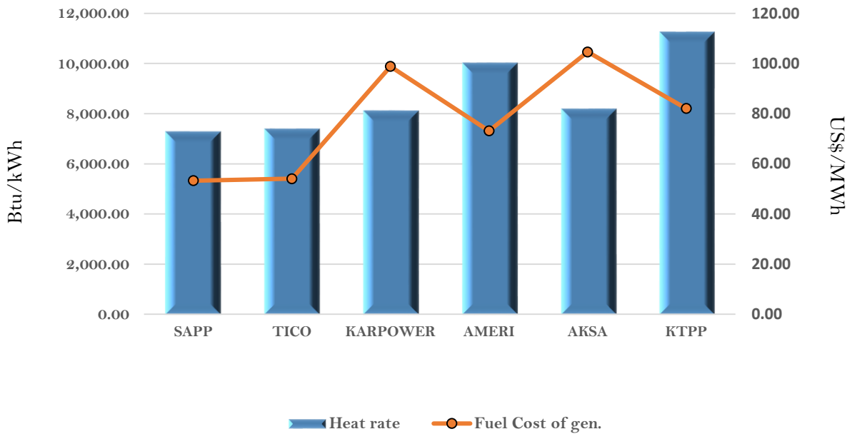
Efficiency and fuel cost of generation on the 31st May 2018
