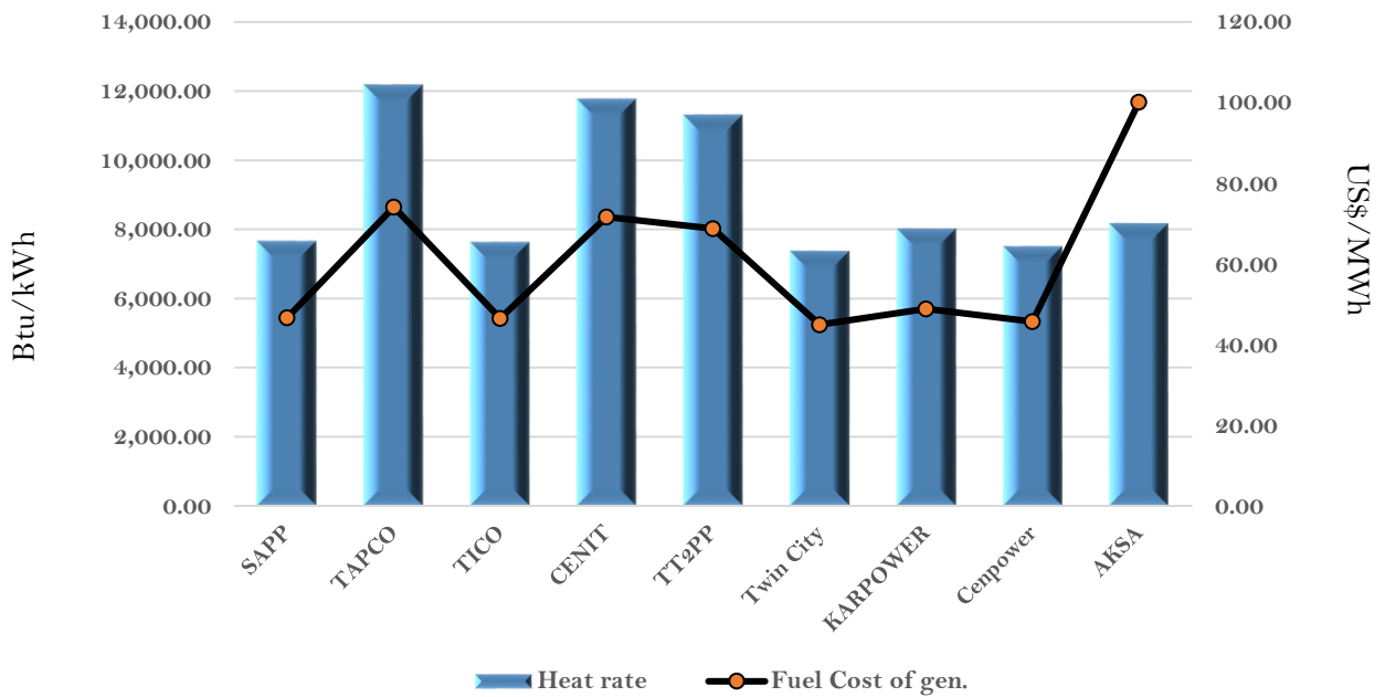
Efficiency and fuel cost of generation on the 28th April 2021
