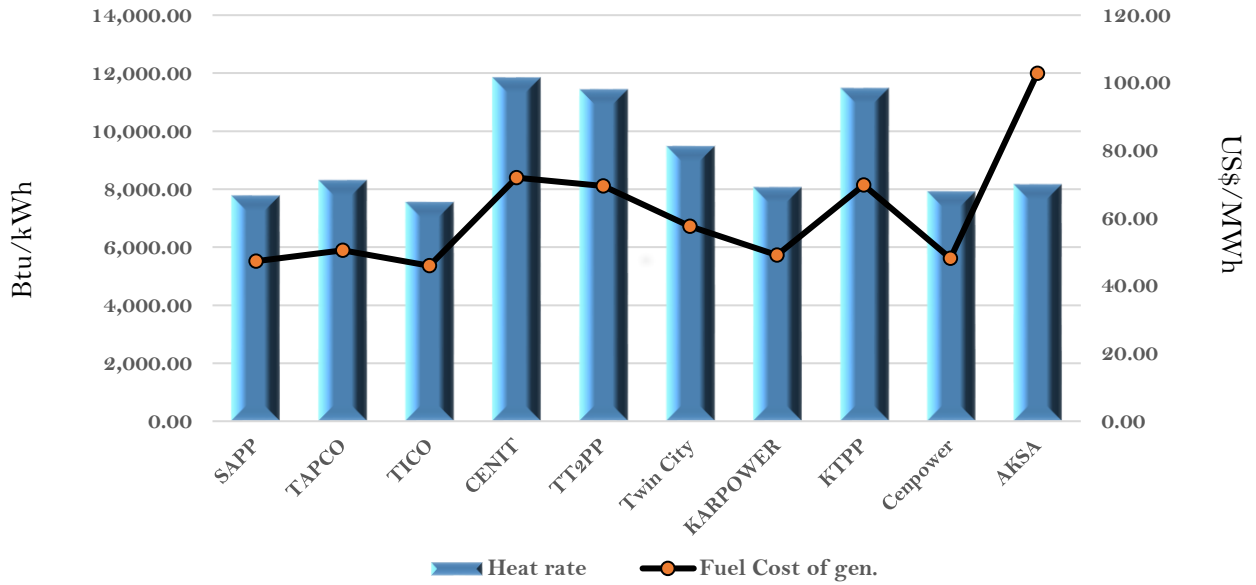
Efficiency and fuel cost of generation on the 29th April 2021
