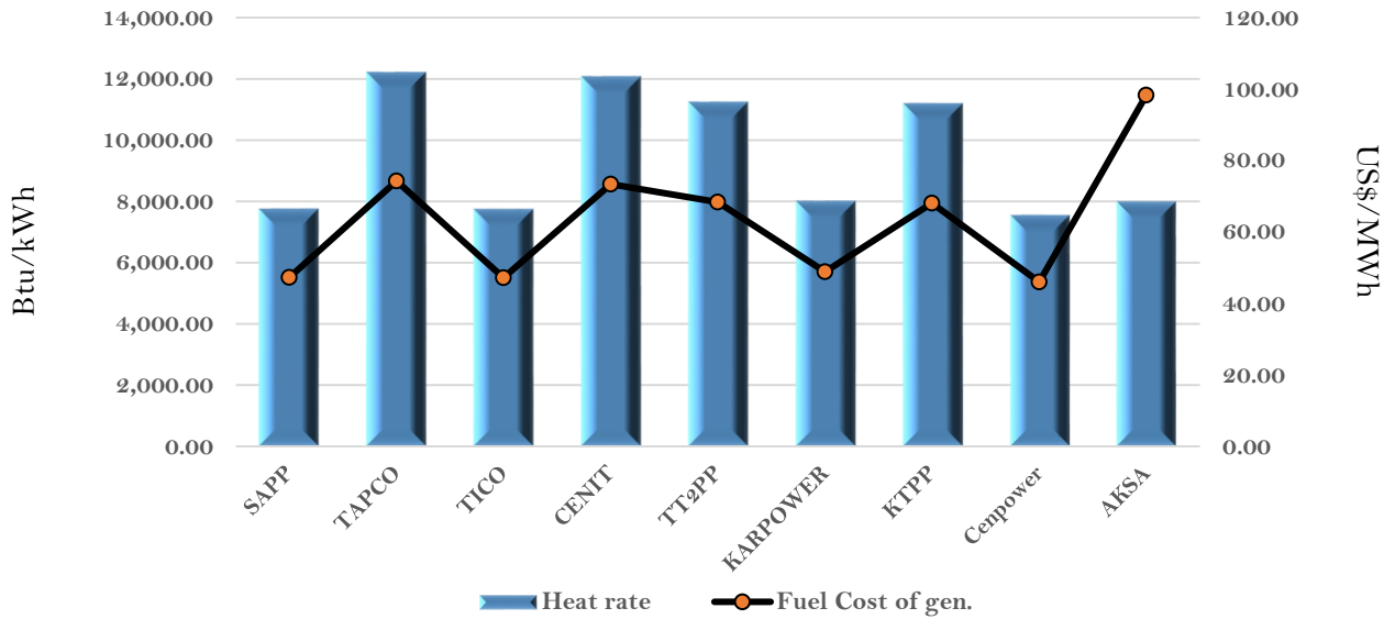
Efficiency and fuel cost of generation on the 23rd April 2021
