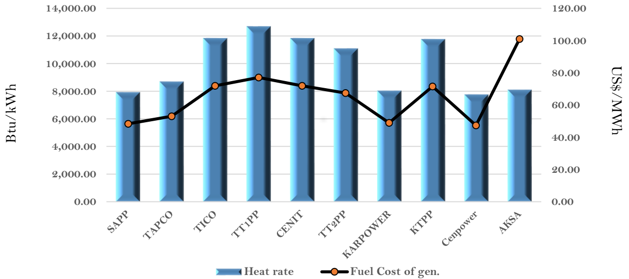
Efficiency and fuel cost of generation on the 30th April 2021
