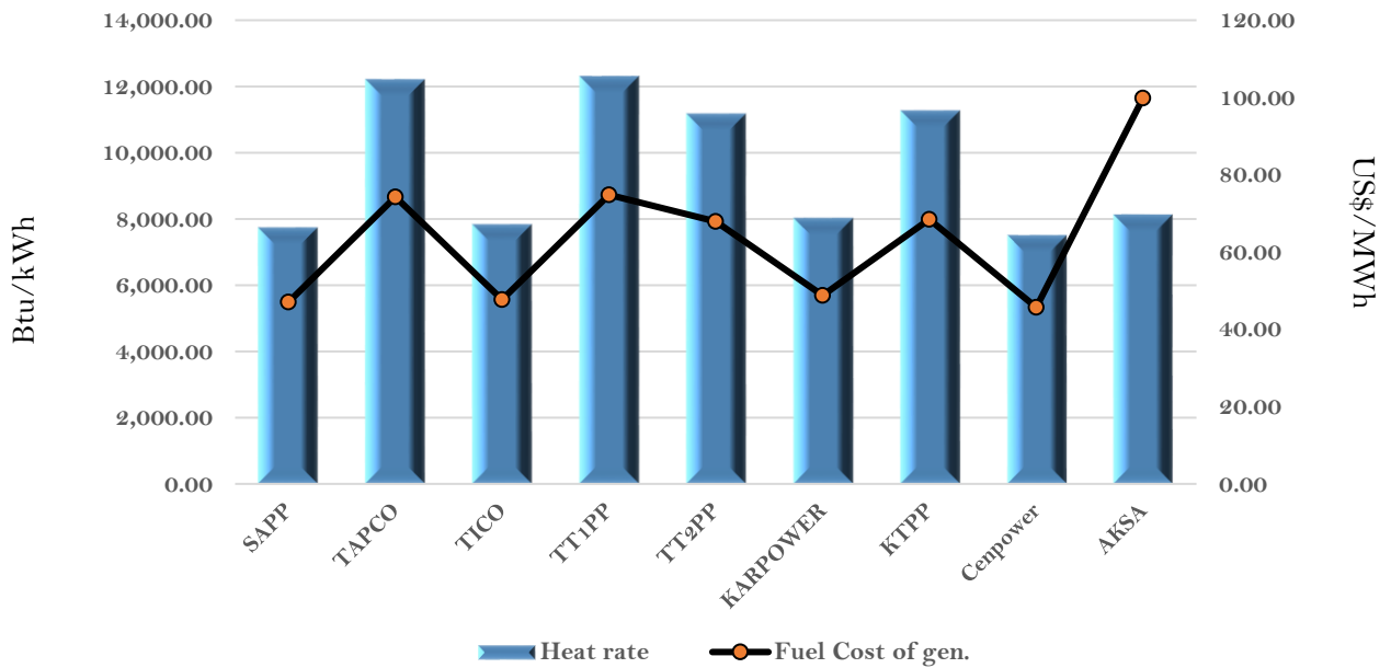
Efficiency and fuel cost of generation on the 24th April 2021
