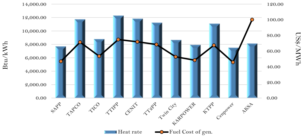
Efficiency and fuel cost of generation on the 27th April 2021
