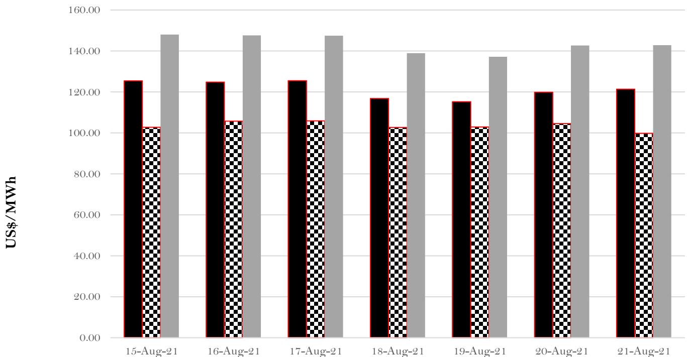
System Marginal Cost Vs Average Market Prices for Week 3 of August 2021
