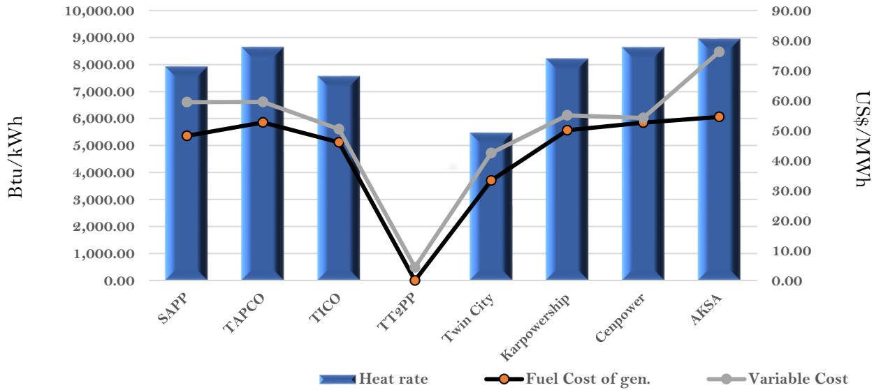
Efficiency and fuel cost of generation on the 18th January 2023
