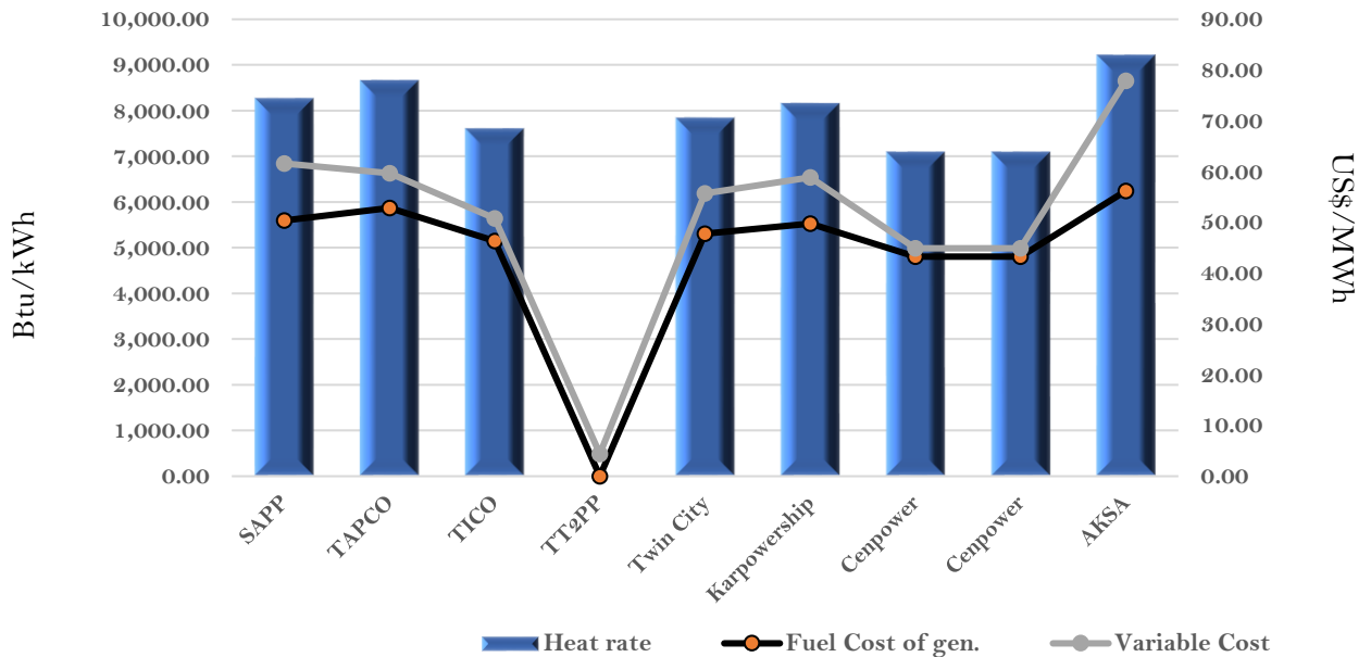
Efficiency and fuel cost of generation on the 19th January 2023
