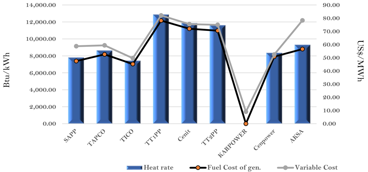
Efficiency and fuel cost of generation on the 6th February 2023
