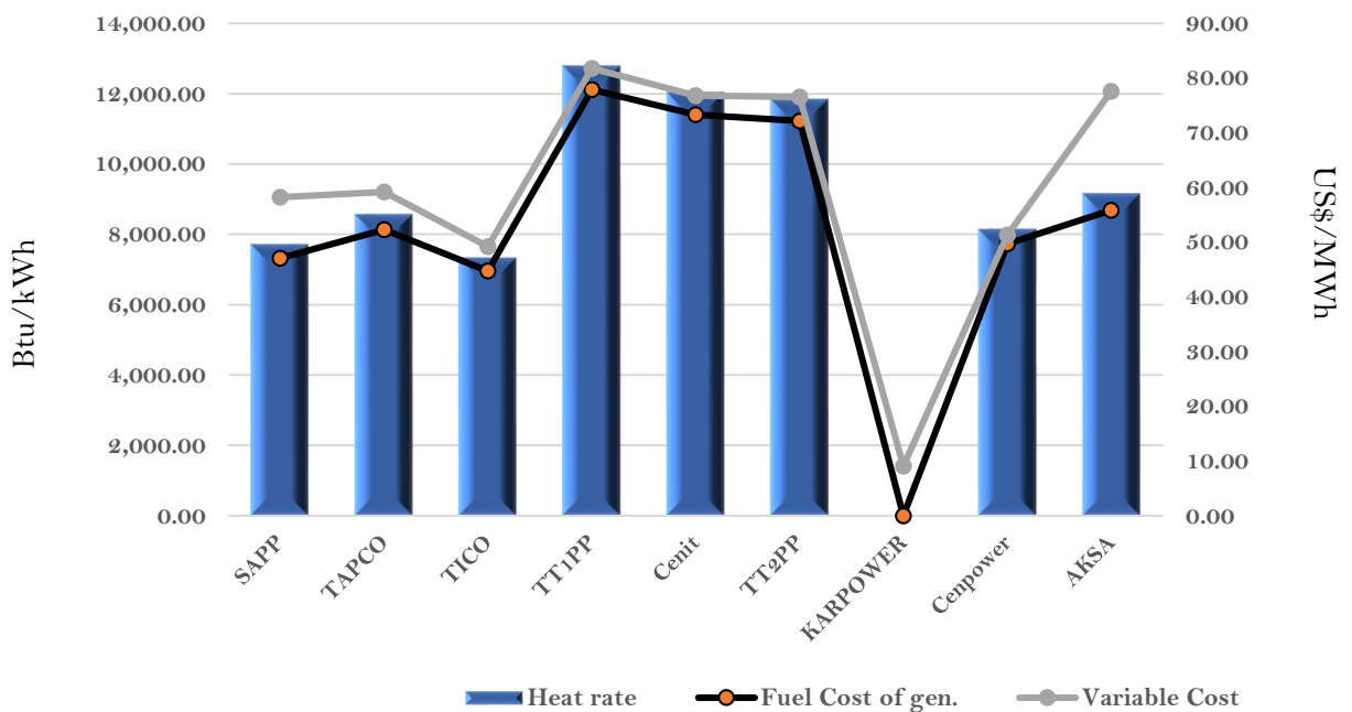
Efficiency and fuel cost of generation on the 7th February 2023
