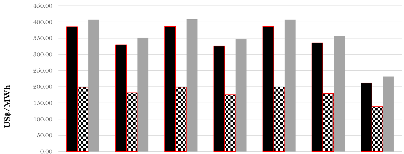
System Marginal Cost Vs Average Market Prices for Week 1 of April 2023
