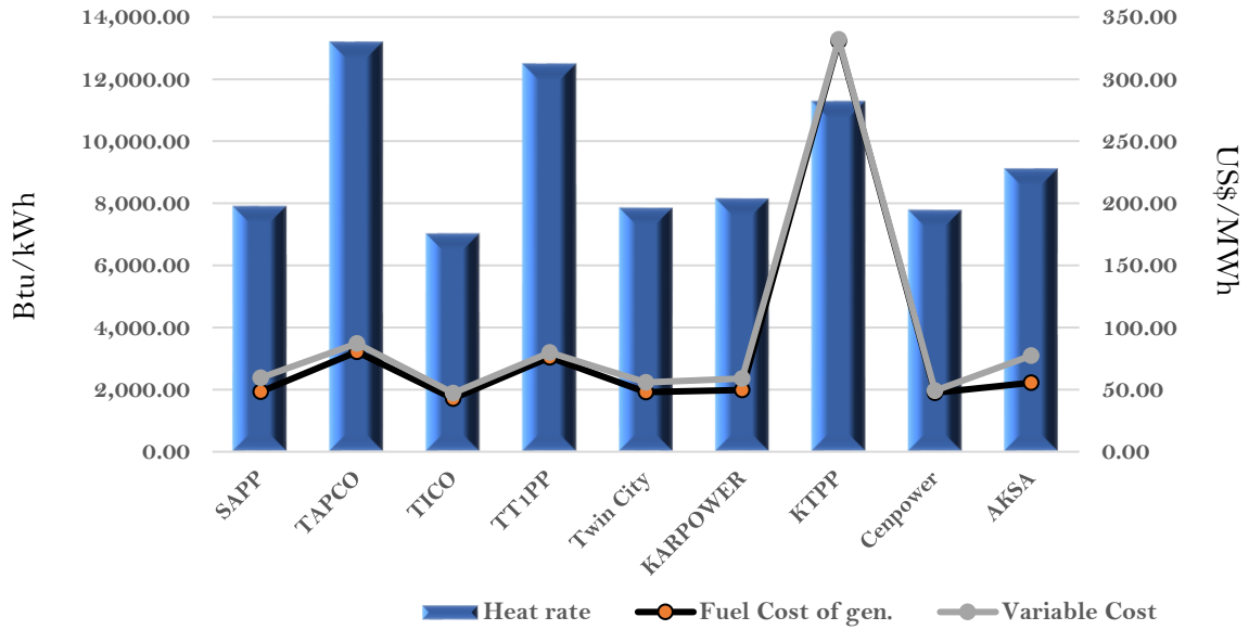
Efficiency and fuel cost of generation on the 13th April 2023
