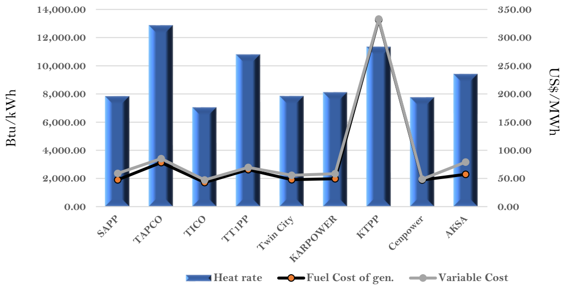
Efficiency and fuel cost of generation on the 14th April 2023
