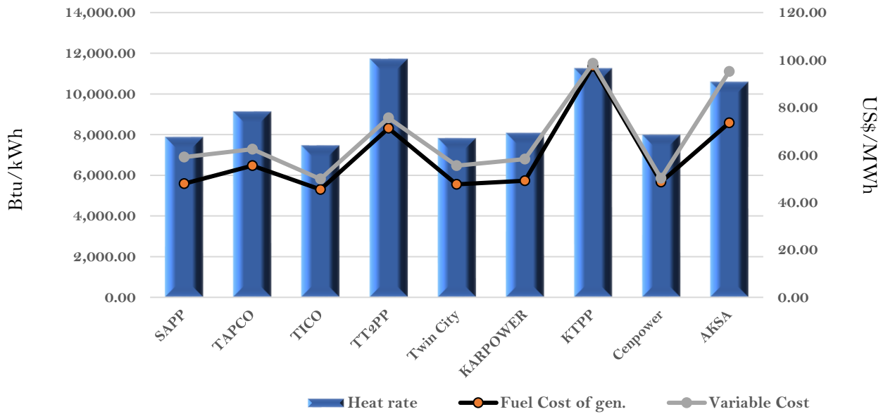
Efficiency and fuel cost of generation on the 11th May 2023
