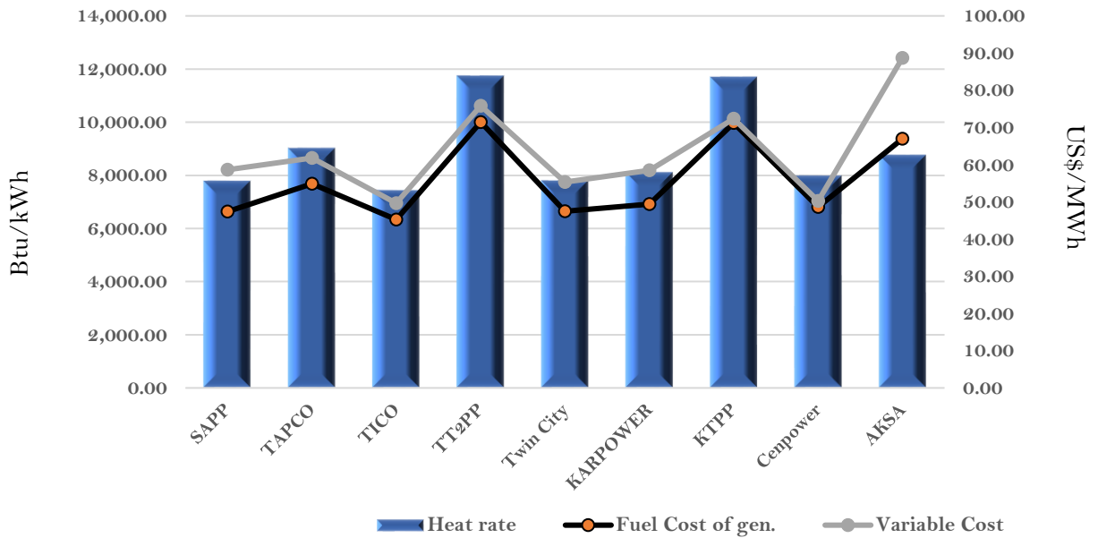
Efficiency and fuel cost of generation on the 13th May 2023
