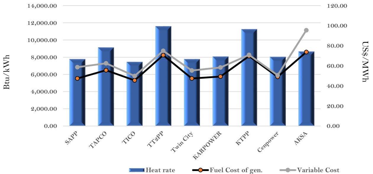
Efficiency and fuel cost of generation on the 12th May 2023
