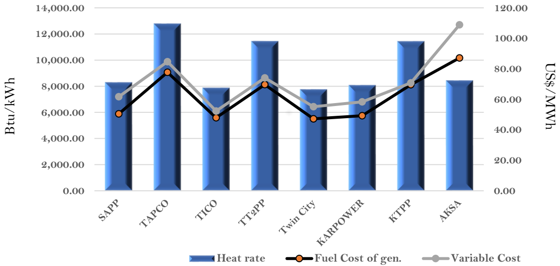
Efficiency and fuel cost of generation on the 6th July 2023
