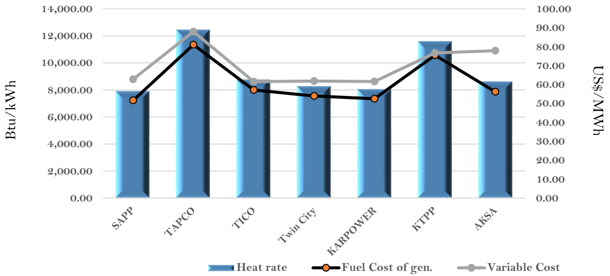
Efficiency and fuel cost of generation on the 13th August 2023
