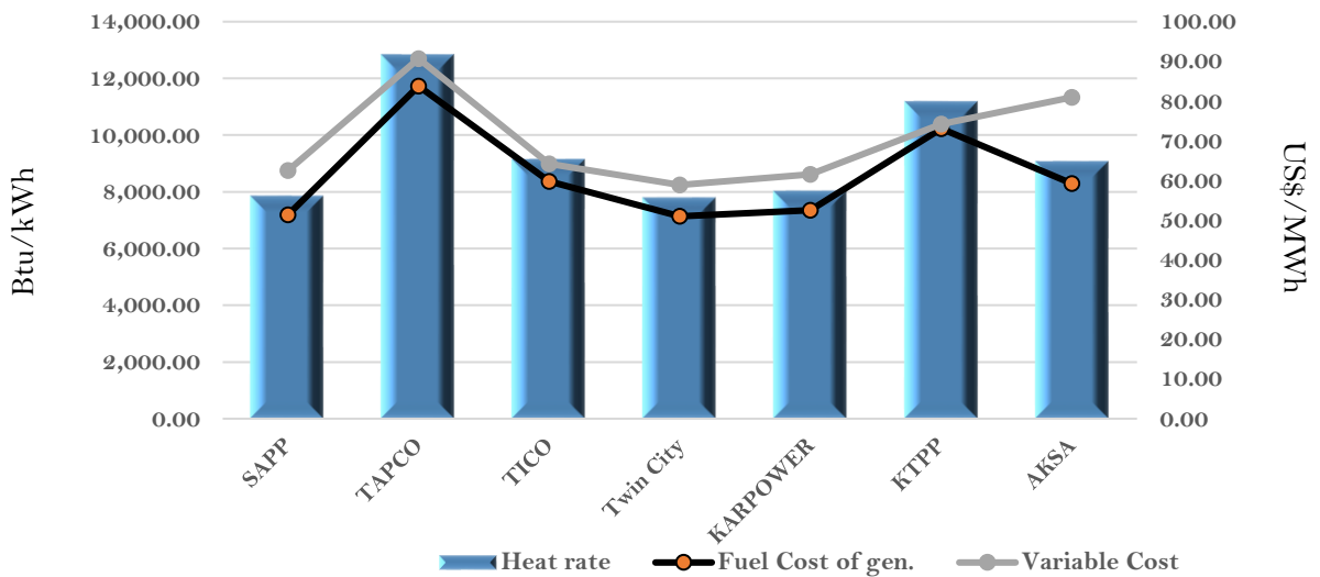
Efficiency and fuel cost of generation on the 14th August 2023
