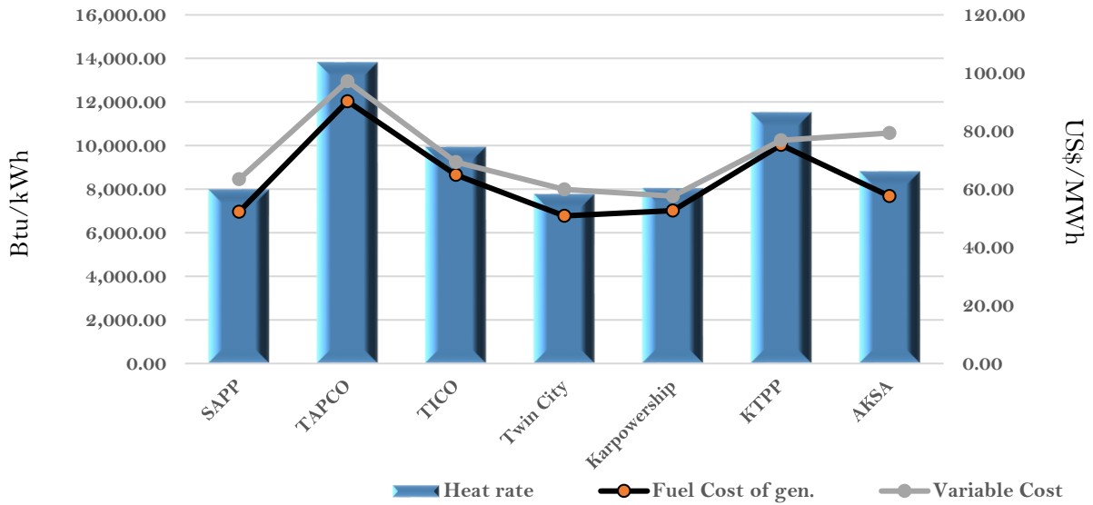
Efficiency and fuel cost of generation on the 18th August 2023
