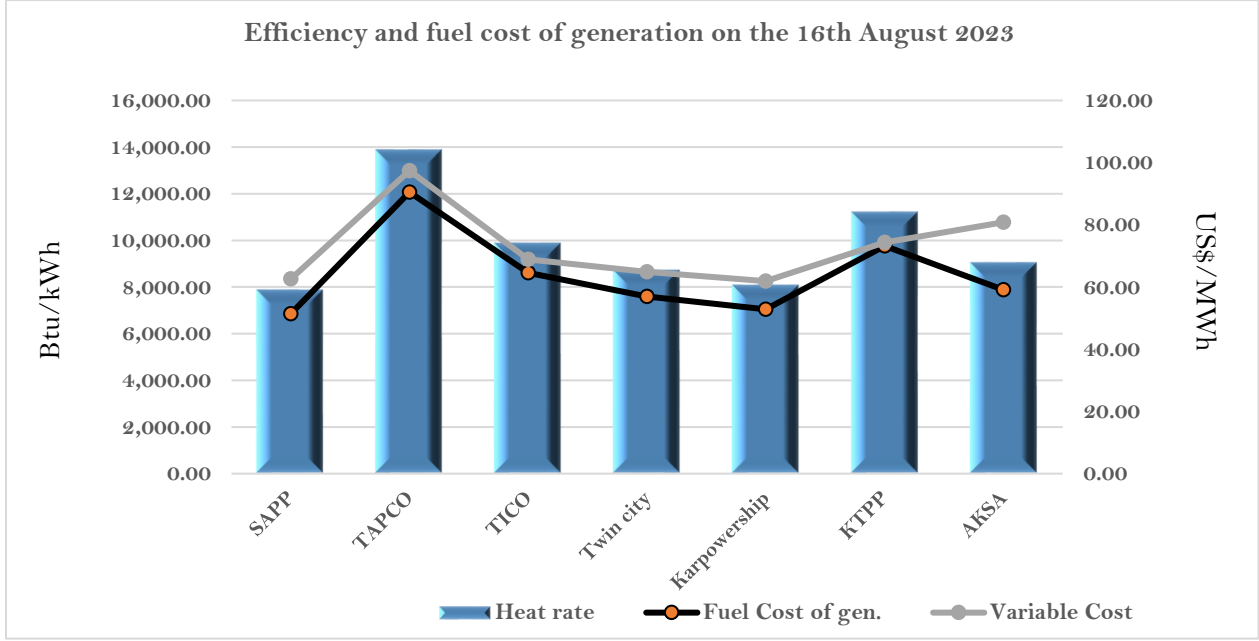
Efficiency and fuel cost of generation on the 17th August 2023
