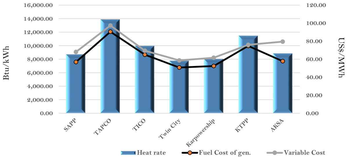
Efficiency and fuel cost of generation on the 19th August 2023
