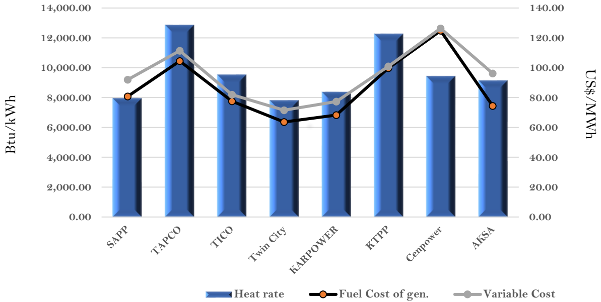
Efficiency and fuel cost of generation on the 7th September 2023
