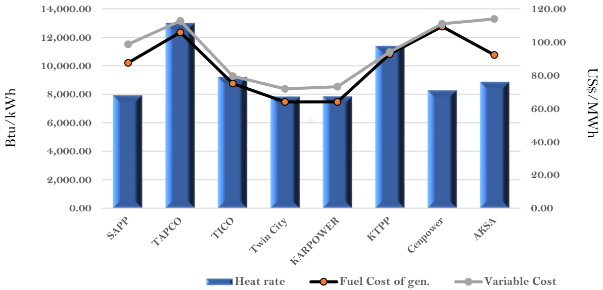
Efficiency and fuel cost of generation on the 7th September 2023
