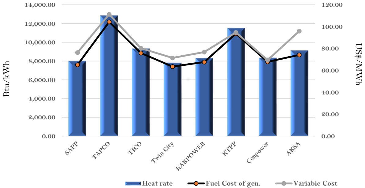
Efficiency and fuel cost of generation on the 2nd September 2023
