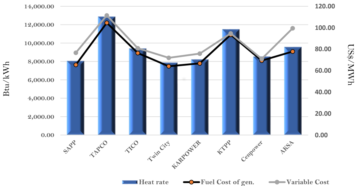
Efficiency and fuel cost of generation on the 3rd September 2023
