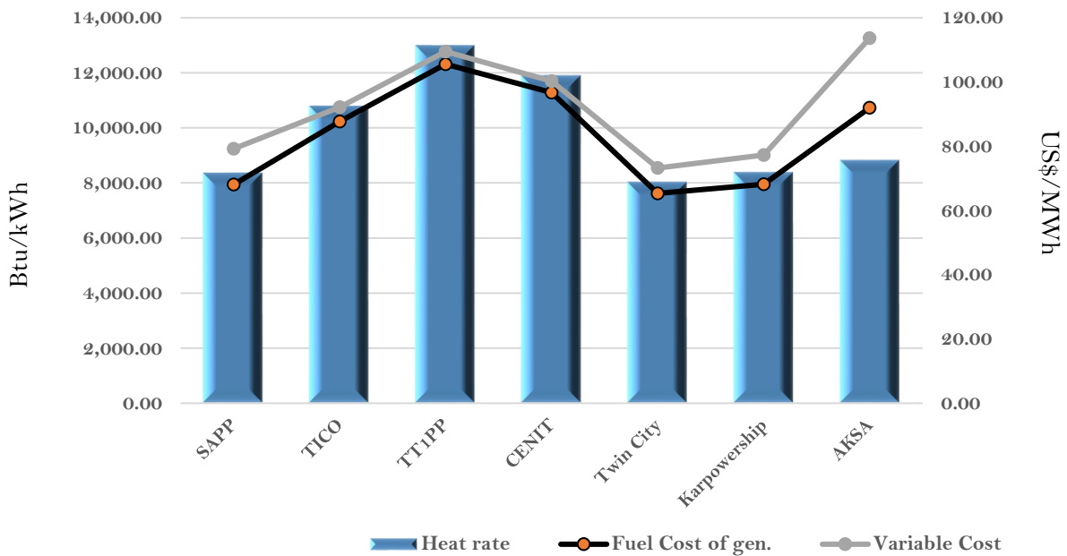
Efficiency and fuel cost of generation on the 19th October 2023
