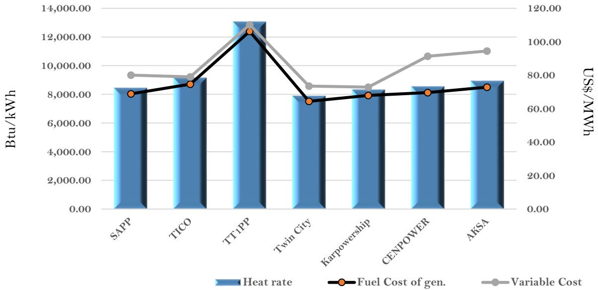
Efficiency and fuel cost of generation on the 19th October 2023
