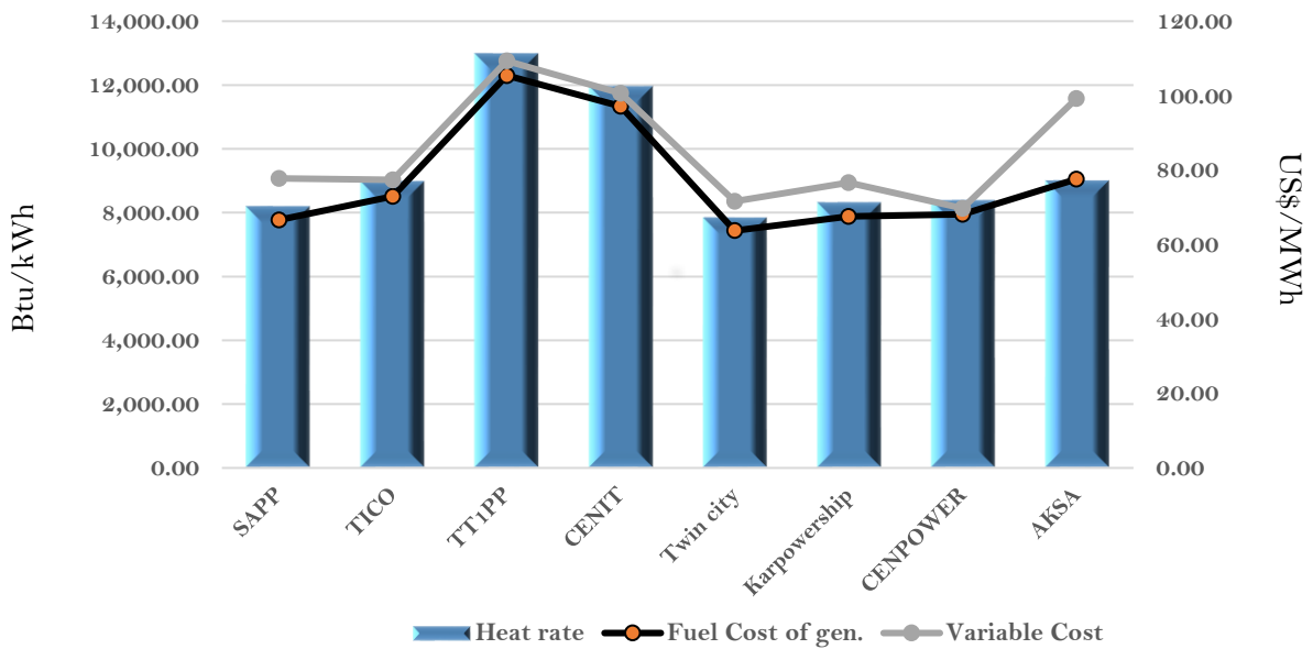
Efficiency and fuel cost of generation on the 17th October 2023
