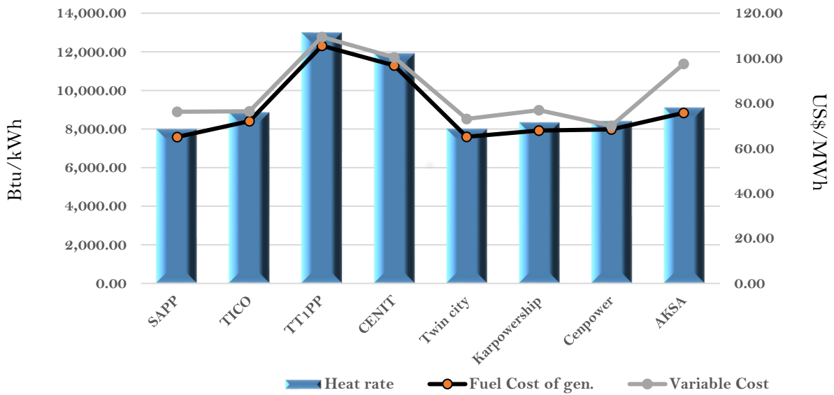
Efficiency and fuel cost of generation on the 17th October 2023
