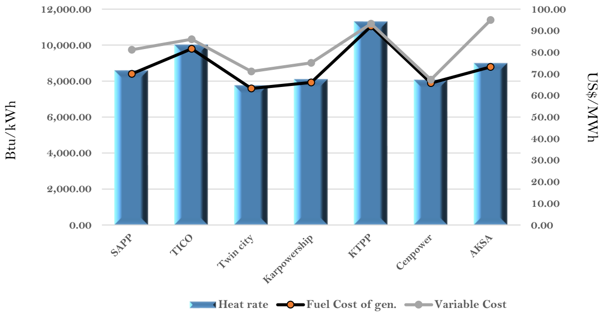
Efficiency and fuel cost of generation on the 17th November 2023
