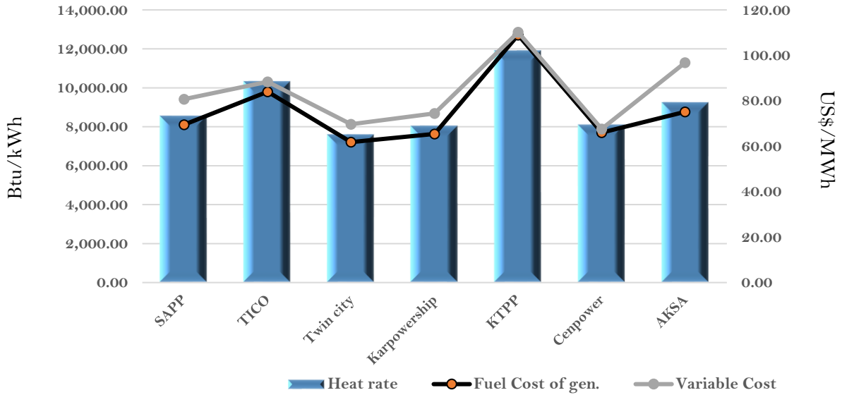
Efficiency and fuel cost of generation on the 17th November 2023
