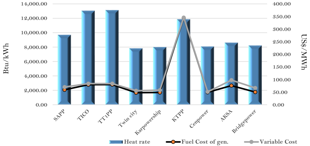
Efficiency and fuel cost of generation on the 30th January 2023
