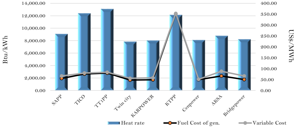
Efficiency and fuel cost of generation on the 31st January 2023
