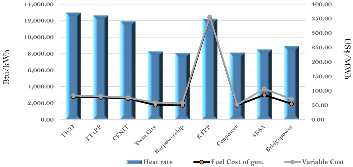
Efficiency and fuel cost of generation on the 24th December 2023
