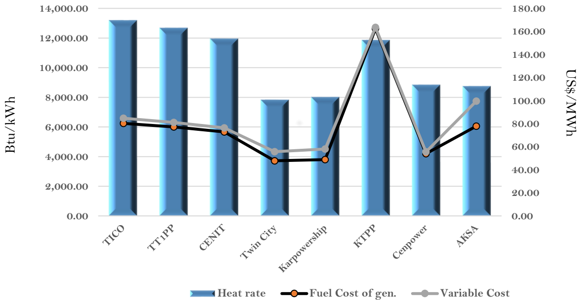
Efficiency and fuel cost of generation on the 24th December 2023
